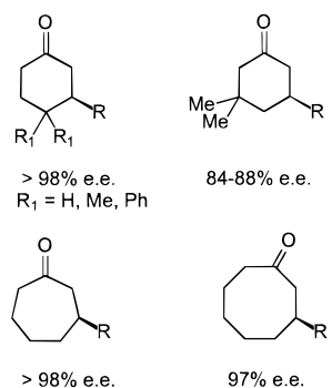
FIGURE 2. Cycloalkanones obtained by enantioselective catalytic 1,4-addition using R_2Zn and catalyst Cu^{II}(OTf)_2/4 . Substituents R are given in Table 1.
